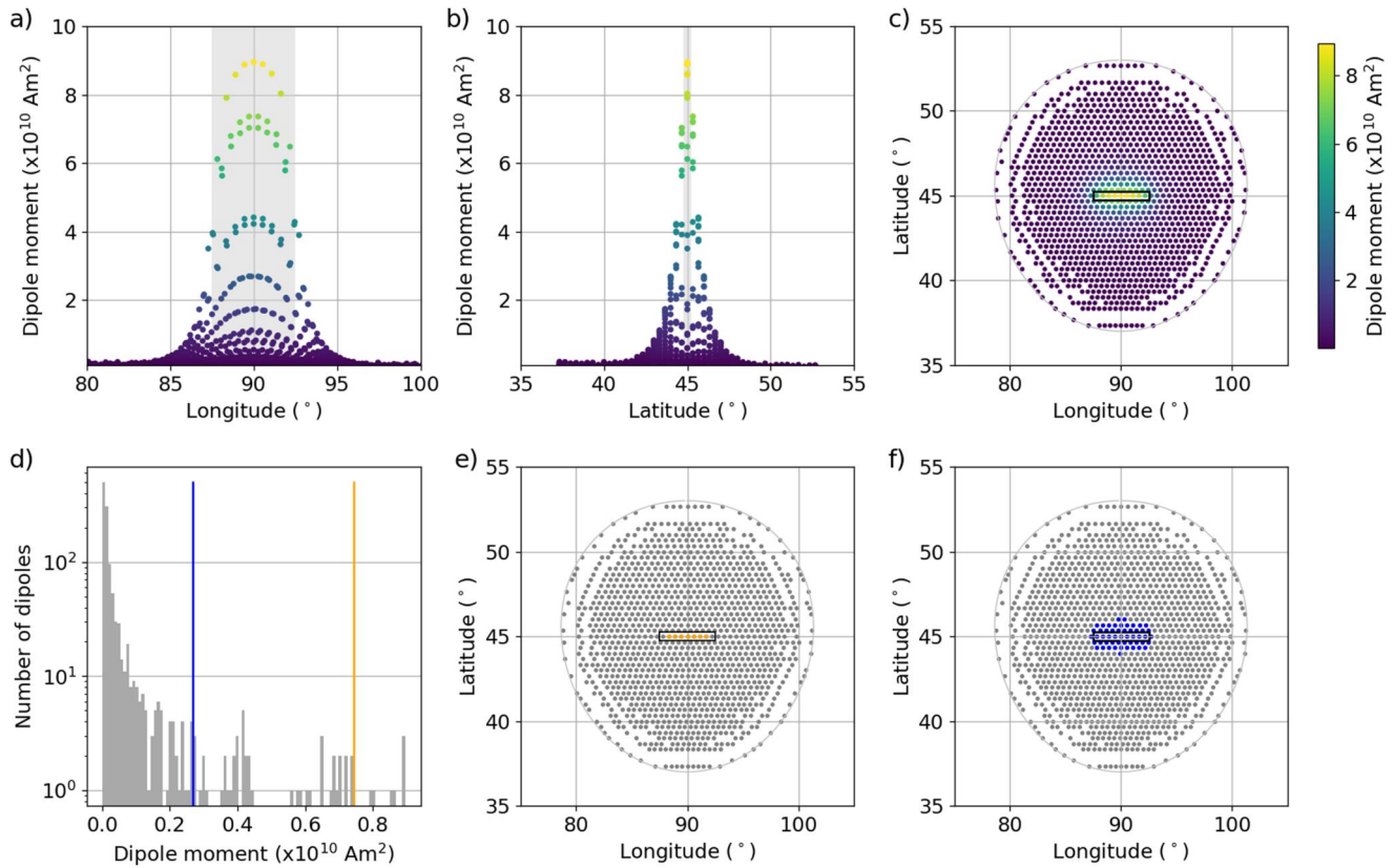
Figure 4. Inversion results of the synthetic magnetized parallelepiped nominal case. All panels are in the same format as Figure 2.
