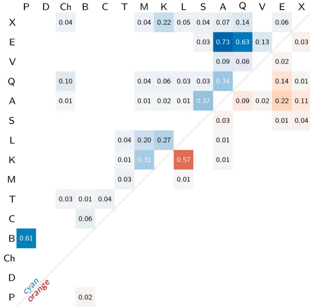
Fig. 7. The two-sample 2 D Kolmogorov-Smirnov p -values estimating the similarity between the observed G_1 , G_2 -pair distributions of the 15 asteroid taxonomic complexes in cyan (upper left) and orange (lower right). Values above 0.2 indicate that the two paired complexes may have the same underlying distribution in G_1 , G_2 -space. Values below 0.01 are not shown for readability. (For interpretation of the references to colour in this figure legend, the reader is referred to the web version of this article.)
