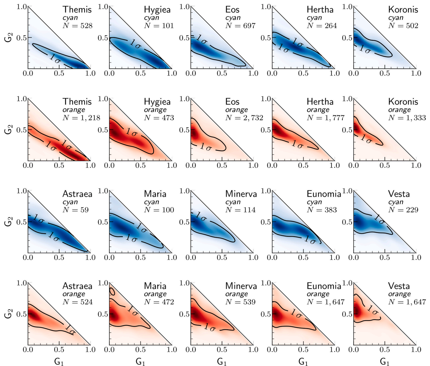
Fig. D.3. Depicted are the G_1, G_2 -distributions of the members of 10 asteroid families observed by ATLAS in cyan (blue) and orange (red). The black contours illustrate the 1 \sigma -levels of the fitted 2 D kernel density estimators. The number of phase curves in each family and band is given by N . (For interpretation of the references to colour in this figure legend, the reader is referred to the web version of this article.)
