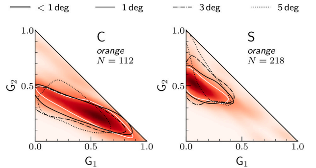
Fig. 12. The effect of insufficient phase curve coverage at low angles on the G_1 , G_2 -parameters. Shown are the 2 D fitted kernel density estimators of the G_1 , G_2 -distribution for C-type and S-type asteroids (red). The solid white line displays the 1 \sigma -level of the distribution using the complete ATLAS phase curves, the black solid, dash-dotted, and dotted contours the distributions using the phase curves truncated at 1 deg., 3 deg., and 5 deg. respectively. (For interpretation of the references to colour in this figure legend, the reader is referred to the web version of this article.)
