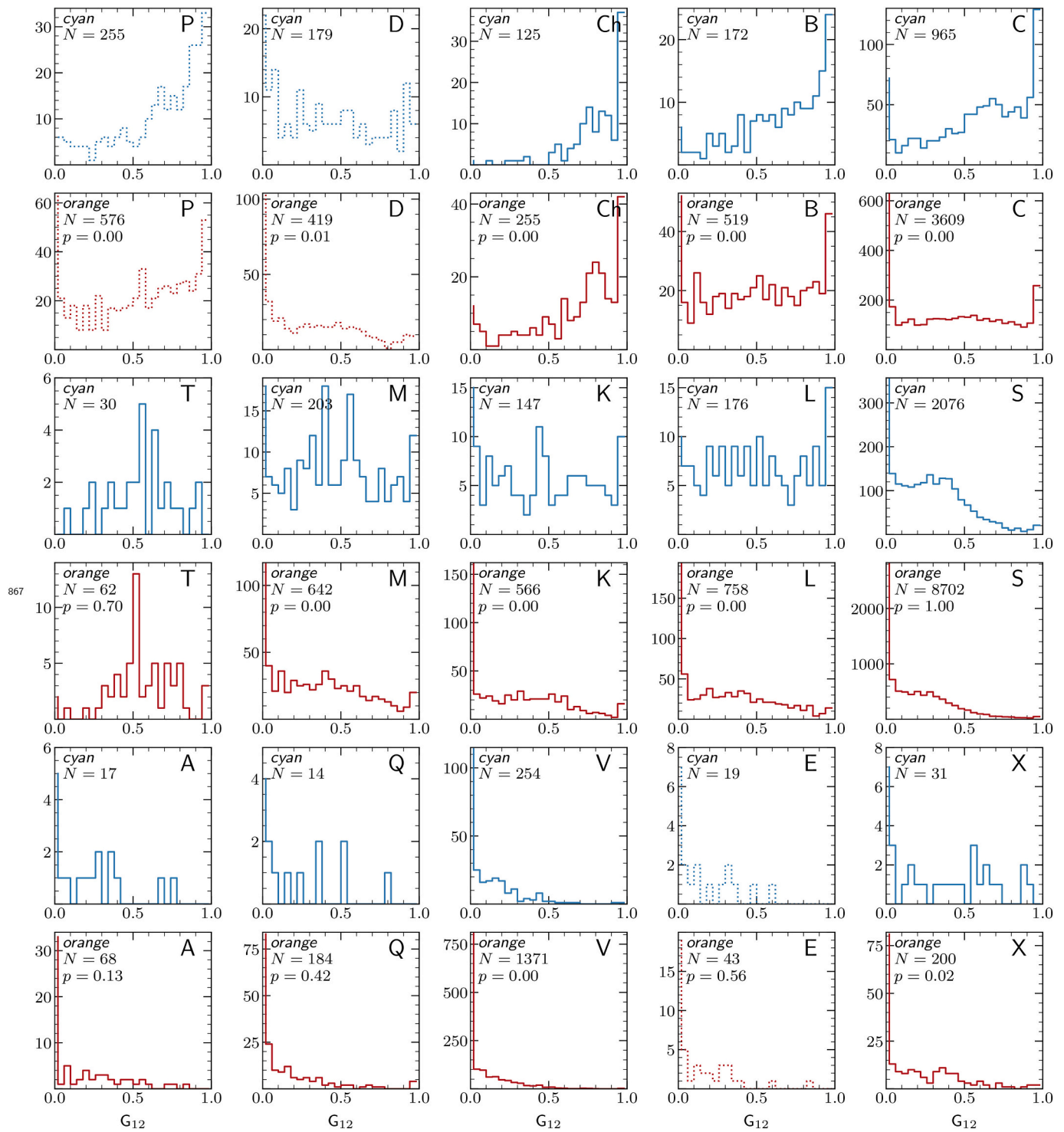
Fig. C.2. The G_{12}^* -distributions for several taxonomic complexes of asteroids, derived from serendipitous observations by ATLAS in cyan and in orange . We give the sample sizes N and the two-sample Kolmogorov-Smirnov p -value between the cyan and orange G_{12}^* -distributions of the complexes. The H , G_{12}^* -model is not suited for the D-, E-, and P-complexes, hence they are displayed with a dotted linestyle. (For interpretation of the references to colour in this figure legend, the reader is referred to the web version of this article.)
