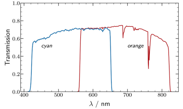
Fig. 1. Transmission curves of the cyan and orange filters used by the ATLAS survey ( Tonry et al., 2018 ). Data from the Filter Profile Service of the Spanish Virtual Observatory ( Rodrigo et al., 2012 ). http://svo2.cab.inta-csic.es/svo/theory/fps3/ . (For interpretation of the references to colour in this figure legend, the reader is referred to the web version of this article.)
