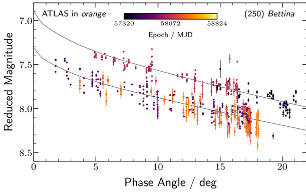
Fig. 10. The phase curve of (250) Bettina as observed by ATLAS in orange. The observations are colour-coded by their epoch, highlighting the four different apparitions that were captured. The triaxial ellipsoid ratios of (250) Bettina are 1.4:1:1 (Viikinkoski et al., 2017). The gray lines show the H , G_1 , G_2 -model fits to the apparitions, split into pairs of two.
