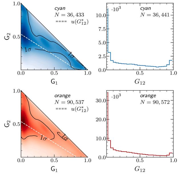
Fig. 5. Left: The 2 D-KDE distribution fitted to the G_1 , G_2 parameters of the phase curves observed in cyan (top) and orange (bottom). The black contours outline the 1 \sigma -levels of the KDE distributions. Right: The histogram of the G_{12}^* -parameter derived from the same sample of phase curves, aligned in the same order. (For interpretation of the references to colour in this figure legend, the reader is referred to the web version of this article.)
