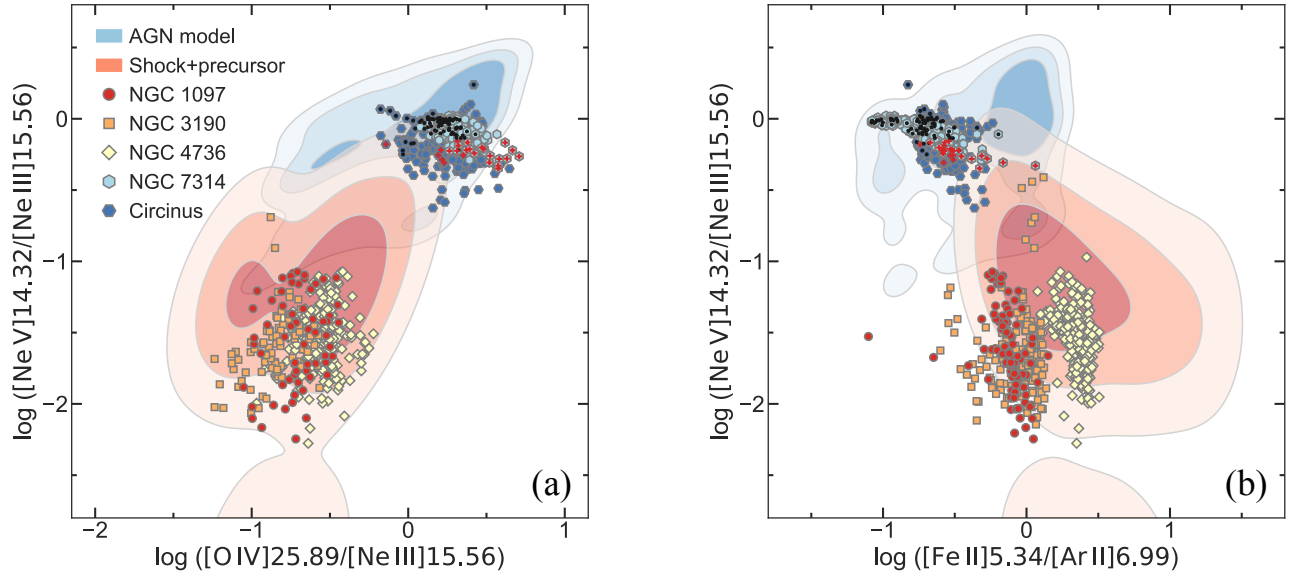
Figure A2. Diagnostic diagrams of ionized emission-line ratios: (a) [\text{Ne V}] 14.32/[\text{Ne III}] 15.56 vs. [\text{O IV}] 25.89/[\text{Ne III}] 15.56 and (b) [\text{Ne V}] 14.32/[\text{Ne III}] 15.56 vs. [\text{Fe II}] 5.34/[\text{Ar II}] 6.99 for 0''.2 \times 0''.2 spaxels in the central \sim 4'' \times 4'' regions of the five AGN targets. The data points with a black circle pertain to spaxels in NGC 7314 and Circinus with \text{PAH } 11.3/7.7 < 0.2 and \text{PAH } 6.2/7.7 < 0.15 , while the points with a red plus sign pertain to those with \text{PAH } 11.3/7.7 > 0.4 . The bluish and reddish contours show the distributions of model results computed by L. Zhang et al. (2025) for AGN and fast radiative shocks (including the shock precursor), respectively. The included AGN models span ionization parameter \log U from -2.3 to -1.8 , AGN spectrum peak energy \log (E_{\text{peak}}/\text{keV}) from -2.1 to -0.9 , metallicities of 1.5\text{--}2 Z_{\odot} , and gas pressure \log (P/k) from 7.0 to 9.5 . The included shock models cover shock velocities v_s from 100 to 400 \text{ km s}^{-1} , pre-shock density n_H from 10^3 to 10^4 \text{ cm}^{-3} , ratio of magnetic to ram pressure \eta_M from 0.0 to 0.001 , and metallicities of 1.5\text{--}2 Z_{\odot} . In each case, the contours enclose 30%, 60%, and 90% of the model results, from the innermost to the outermost levels. Note that some spaxels have valid [\text{Ne V}] 14.32 \mu\text{m} measurements from Ch3 but no corresponding [\text{O IV}] 25.89 \mu\text{m} measurements from Ch4; consequently, panel (a) contains fewer data points than panel (b).
