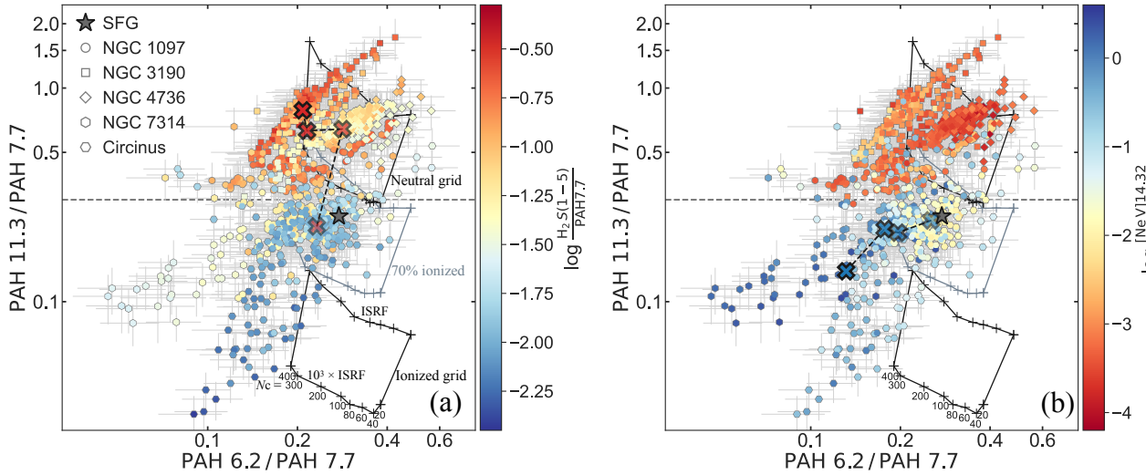
Figure 4. PAH band ratio diagrams for 0''.2 \times 0''.2 spaxels in the central \sim 4'' \times 4'' regions of the five AGN targets, color-coded by the strength indicators of (a) shock processing ( r_{H_2} ) and (b) AGN irradiation ( r_{Ne} ). The horizontal dashed lines mark the empirical demarcation at PAH\ 11.3/7.7 = 0.3 . The reddish and bluish crosses in panels (a) and (b) show, for the five AGN targets, the median PAH band ratios of the spaxels in bins of increasing \log(r_{H_2}) of [-2, -1.5] , [-1.5, -1.0] , [-1.0, -0.5] , and [-0.5, 0] , and increasing \log(r_{Ne}) of [-2, -1.5] , [-1.5, -0.75] , [-0.75, 0] , and [0, 0.5] (from light to dark), respectively. The gray star labeled “SFG” represents the median PAH band ratios of the spatially resolved spaxels in star-forming galaxies measured by L. Zhang et al. (2022); the individual star formation spaxels, which are clustered around the median value, are omitted for clarity. The grids marked by a plus sign in each panel show model predictions of PAH band ratios from D. Rigopoulou et al. (2024) for neutral (top grids), 70% ionized (middle grids), and fully ionized (bottom grids) PAHs of various sizes (carbon number N_C = 20\text{--}400 , increasing from the right to the left boundary of each grid). The grids span the interstellar radiation field (ISRF; top boundary) up to 10^3 \times ISRF (bottom boundary).
