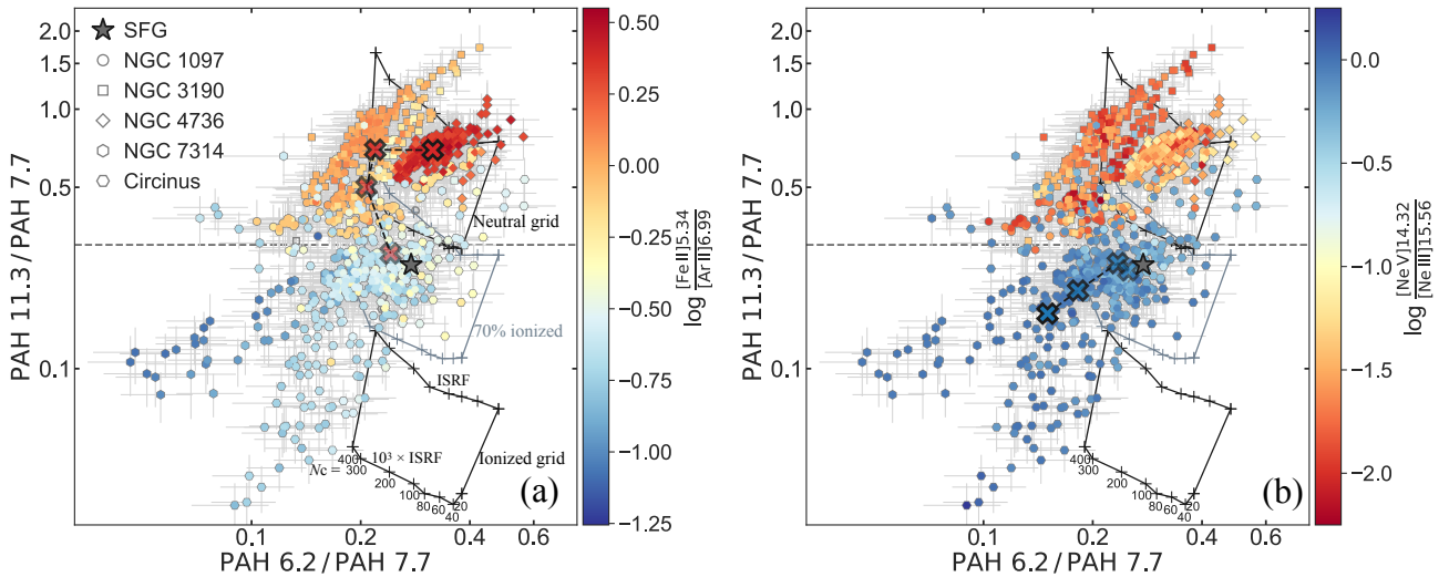
Figure 5. Same as Figure 4, but color-coded by the different strength indicators of (a) shock processing ( [\text{Fe II}] 5.34/[\text{Ar II}] 6.99 ) and (b) AGN irradiation ( [\text{Ne V}] 14.32/[\text{Ne III}] 15.56 ). The reddish and bluish crosses in panels (a) and (b) show, for the five AGN targets, the median PAH band ratios of the spaxels in bins of increasing \log ([\text{Fe II}] 5.34/[\text{Ar II}] 6.99) of [-0.5, -0.25] , [-0.25, 0] , [0, 0.25] , and [0.25, 0.5] and increasing \log ([\text{Ne V}] 14.32/[\text{Ne III}] 15.56) of [-0.5, -0.3] , [-0.3, -0.15] , [-0.15, 0] , and [0, 0.2] (from light to dark), respectively.
