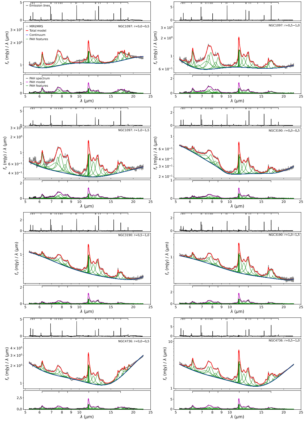
Figure A4. Top panels: emission-line spectra obtained by subtracting the PAH emission and underlying continuum (i.e., the red curves in the middle panels) from the integrated MIRI/MRS spectra extracted from the r \leq 0\farcs5 , 0\farcs5 \leq r \leq 1\farcs0 , and 1\farcs0 \leq r \leq 1\farcs5 regions of each target. From left to right, the short markers at the top indicate the positions of the [Fe II] 5.34 \mu\text{m} , [Fe VIII] 5.45 \mu\text{m} , [Mg VII] 5.50 \mu\text{m} , [Mg V] 5.61 \mu\text{m} , \text{H}_2 S(6), \text{H}_2 S(5), [Ar II] 6.985 \mu\text{m} , [Na III] 7.32 \mu\text{m} , \text{P}\alpha , [Ne VI] 7.65 \mu\text{m} , [Fe VII] 7.815 \mu\text{m} , [Ar V] 7.90 \mu\text{m} , \text{H}_2 S(4), [Ar III] 8.99 \mu\text{m} , [Fe VII] 9.53 \mu\text{m} , \text{H}_2 S(3), [S IV] 10.51 \mu\text{m} , \text{H}_2 S(2), \text{H}\alpha , [Ne II] 12.81 \mu\text{m} , [Ar V] 13.10 \mu\text{m} , [Ne V] 14.32 \mu\text{m} , [Ne III] 15.555 \mu\text{m} , \text{H}_2 S(1), and [S III] 18.71 \mu\text{m} emission lines. Middle panels: illustrations of the multicomponent fitting procedure used for the PAH measurements (see Section 2.3). The gray curves show the observed MIRI/MRS spectra with emission lines masked. The red curves represent the best-fit models consisting of PAH emission and the underlying continuum. The blue curves show the combined underlying continuum components (i.e., stellar and dust continua), while the green curves represent the individual PAH features modeled with Drude profiles. Bottom panels: PAH spectra (black curves) obtained by subtracting all continuum components (i.e., the blue curves in the middle panels) from the emission-line-masked MIRI/MRS spectra. As in the middle panels, the green curves represent individual PAH features modeled with Drude profiles, while the magenta curves show their sum, corresponding to the modeled PAH spectra. From left to right, the short markers at the top indicate the positions of the PAH complexes centered near 6.2 , 7.7 , 8.6 , 11.3 , 12.7 , and 17.0 \mu\text{m} . Note that all x -axes, as well as the y -axes in the middle panels, are shown on logarithmic scales, whereas the y -axes in the top and bottom panels are shown on linear scales. No spectrum is shown for the r \leq 0\farcs5 region of Circinus, as noted in Figure A3.
