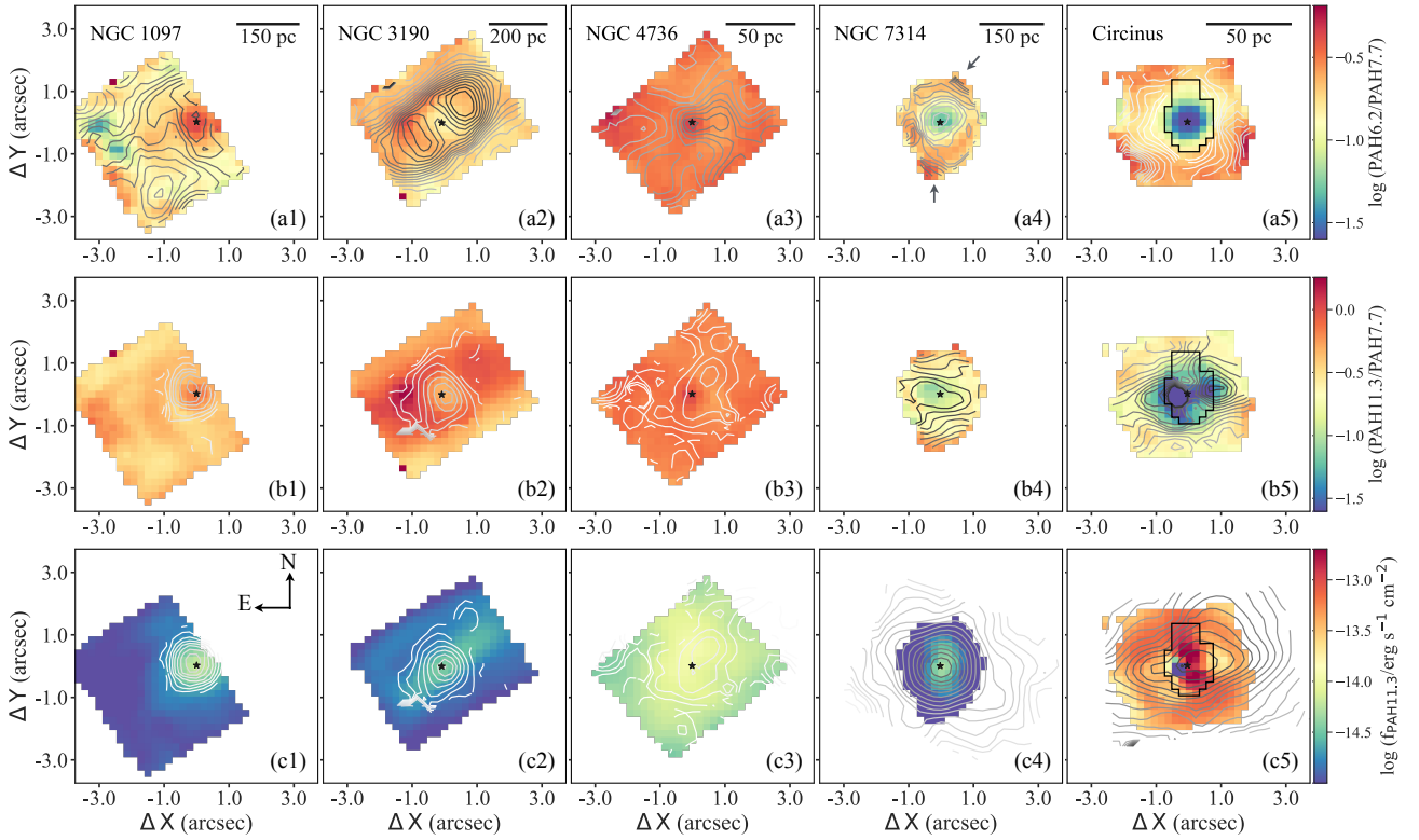
Figure 3. Spatially resolved maps of PAH 6.2/7.7 ratio (top panels), PAH 11.3/7.7 ratio (middle panels), and PAH 11.3 \mu\text{m} emission (bottom panels) for the five AGN targets. Each column corresponds to one target, with the AGN position denoted by a black star. A common color scale is adopted for all panels within a given row and is shown on the right. The contours in the top, middle, and bottom panels show the distributions of \log(r\text{H}_2) ( -2.25 to -0.5 ), \log(r\text{Ne}) ( -4.0 to 0.15 ), and \log(f_{\text{[Ne III]}} 14.32 \mu\text{m}/\text{erg s}^{-1} \text{cm}^{-2}) ( -18.0 to -13.3 ), respectively, with higher values indicated by darker colors on a common scale for each row. The black arrows in panel (a4) indicate the locations of the two radio spots in NGC 7314. The black polygons in Circinus outline the region within which the spaxels are shown here for illustrative purposes; these spaxels are excluded from the statistical analyses owing to the lack of reliable spaxel-based measurements of [Ne III] 15.56 \mu\text{m} and/or H 2 S(1) and S(2), as detailed in Section 2.2. North is up in all panels, and the physical scale of each target is labeled in the upper right corner of each top panel.
