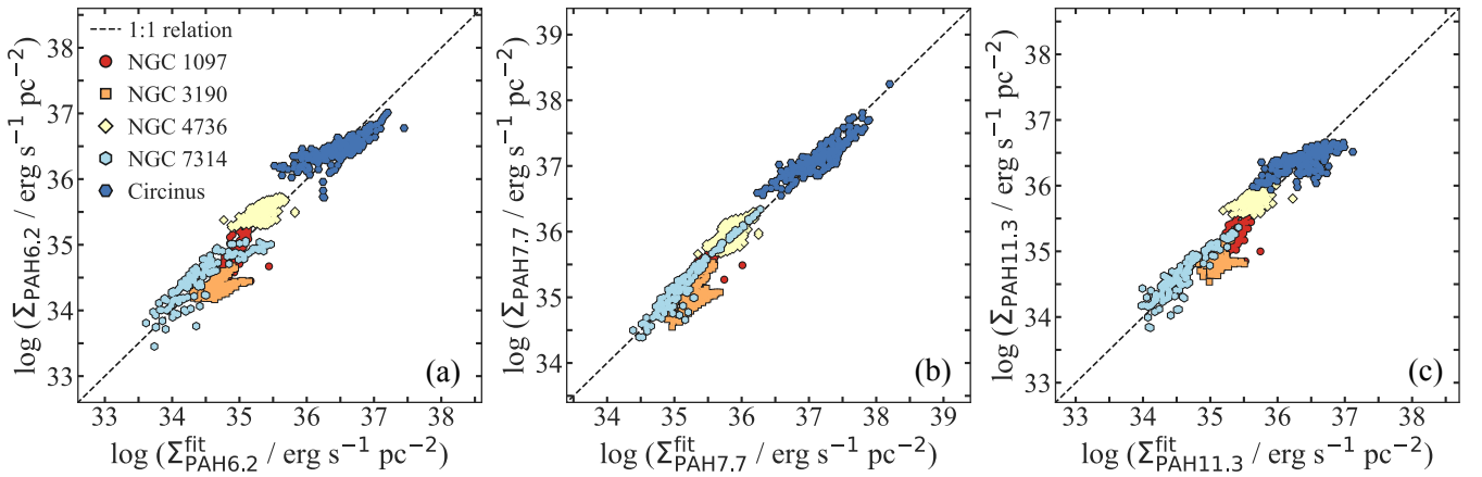
Figure 2. Correlations between the surface brightness of the measured PAH (a) 6.2 \mu\text{m} , (b) 7.7 \mu\text{m} , and (c) 11.3 \mu\text{m} emission and those predicted by Equation (1) for data points in Figure 1, with the dashed line in each panel indicating the 1:1 relation.
