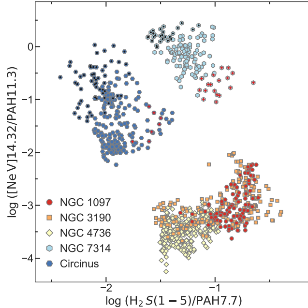
Figure A1. Diagnostic diagram of [Ne V] 14.32/PAH 11.3 (i.e., rNe) vs. H_2 S(1-5)/PAH 7.7 (i.e., rH 2 ) for 0''.2 \times 0''.2 spaxels in the central \sim 4'' \times 4'' regions of the five AGN targets. The data points highlighted with black circles pertain to spaxels in NGC 7314 and Circinus with PAH 11.3/7.7 < 0.2 and PAH 6.2/7.7 < 0.15, while the points highlighted with red plus signs pertain to those with PAH 11.3/7.7 > 0.4.
